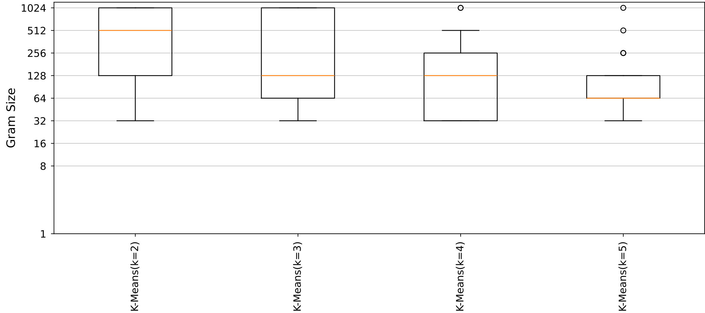
YARA Rules Gram Size Distribution (Cluster36_Size5 dataset)
